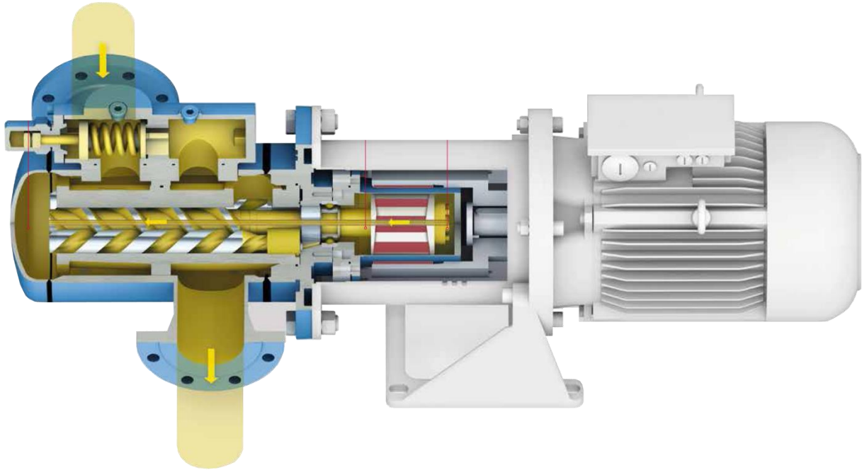
KRAL API Pumpe
